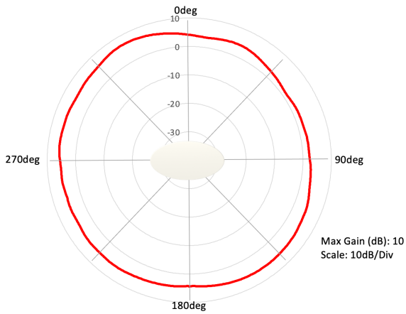
2.4 GHz Azimuth
